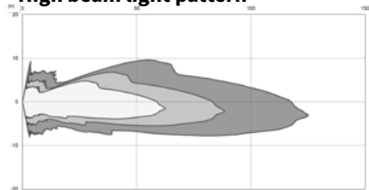
Low beam light pattern
